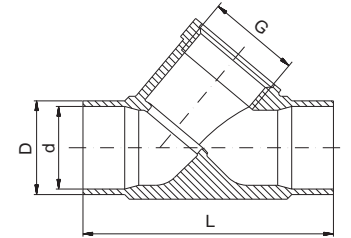
Anschweißenden ISO 4200 "L" / welded connection ISO 4200 "L"
