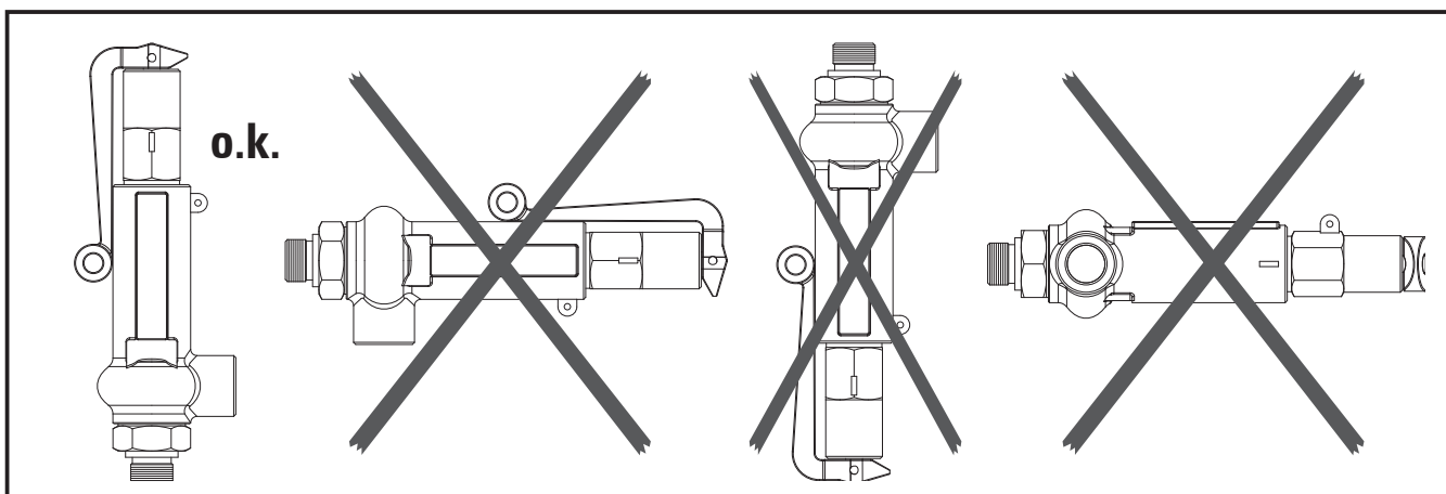
Fig.4.1 - Safety Valves, Installation (Fig. shows Art. NG301023 with head „A“)
