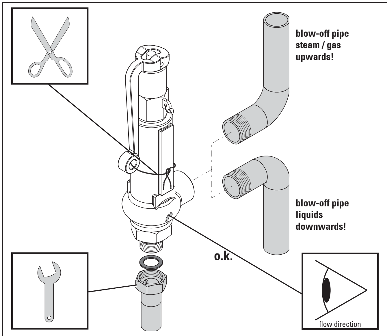
Fig. 4.2 - Safety Valves, Mounting with threaded connection (Fig. shows Art. NG301023 with head „A“)
