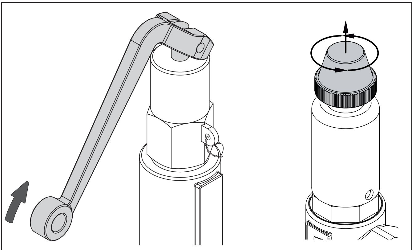
Fig. 4.3 - Safety Valve, Operating of the ventilation
