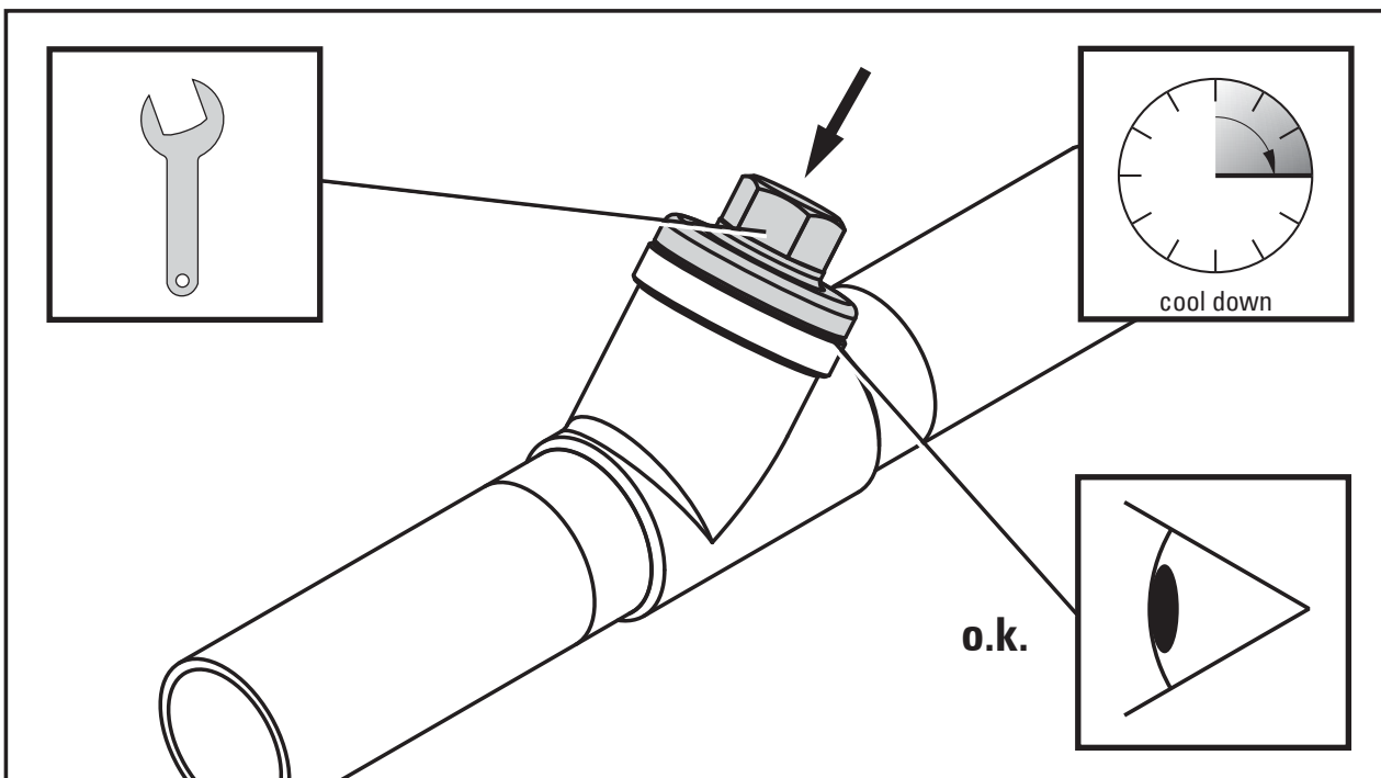
Fig. 5.5 - non-return valve, swing-check valve, mounting of the bonnet and the inner parts (Fig.: Art. EB310064)
