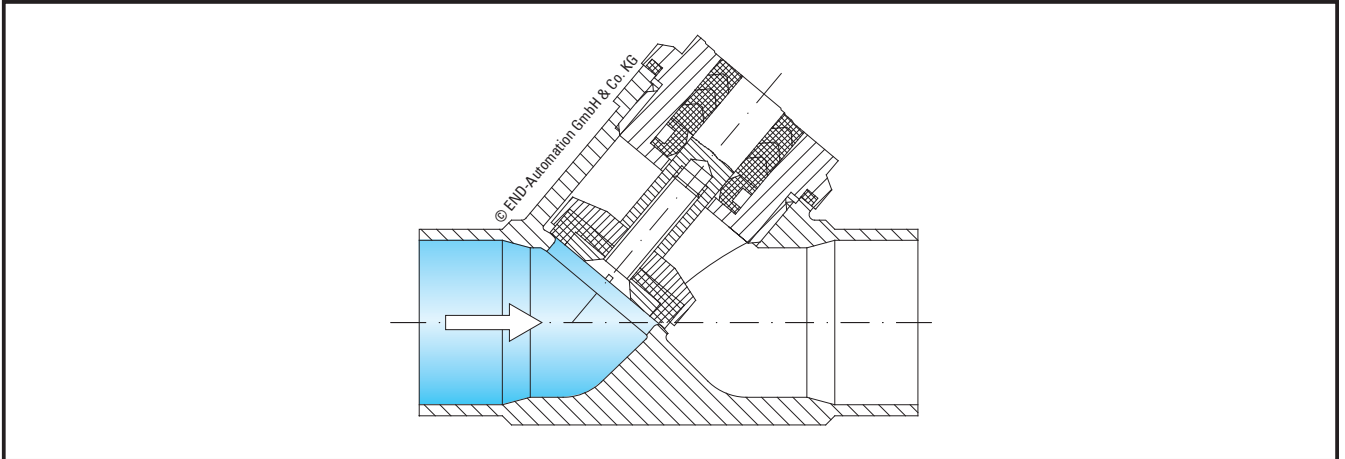
Fig. 4.6 - Description of function - Normally close against the flow direction
